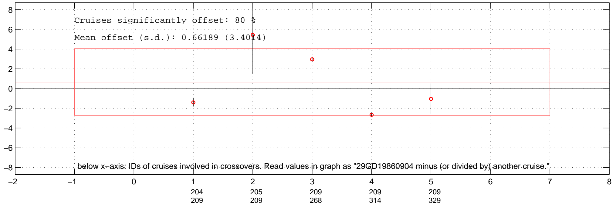
all additive offsets of ALK of 29GD19860904 in Favourite-space.
