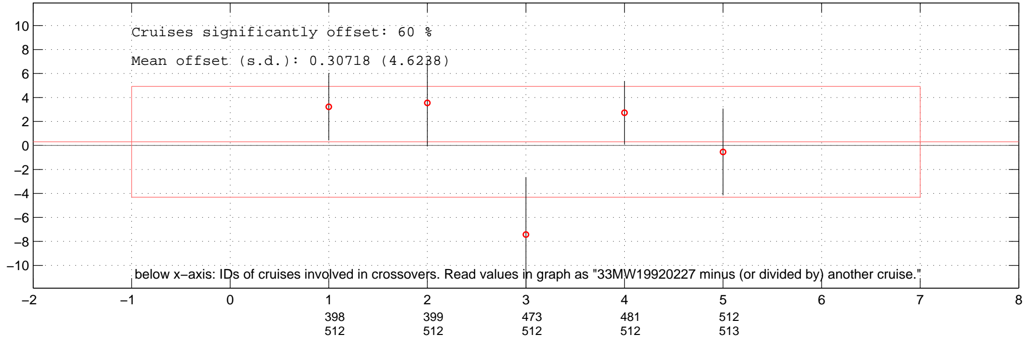
all additive offsets of ALK of 33MW19920227 in Favourite-space.
