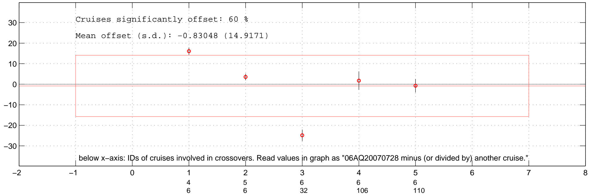
all additive offsets of ALK of 06AQ20070728 in Favourite-space.
