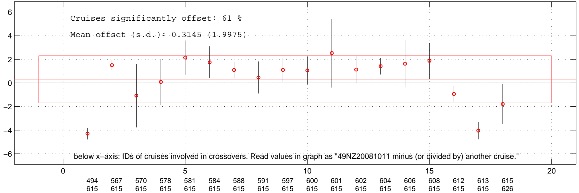
all additive offsets of ALK of 49NZ20081011 in Favourite-space.
