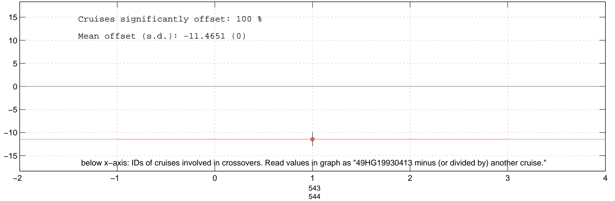
all additive offsets of ALK of 49HG19930413 in Favourite-space.
