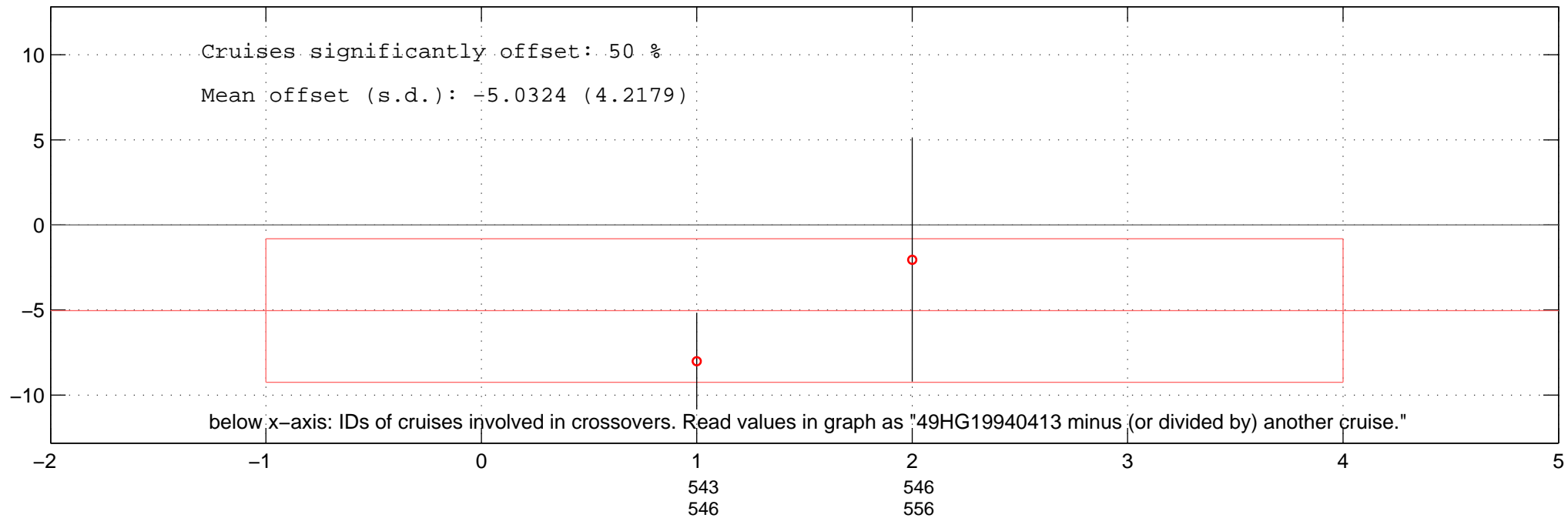
all additive offsets of ALK of 49HG19940413 in Favourite-space.
