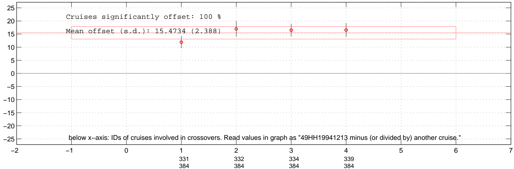
all additive offsets of ALK of 49HH19941213 in Favourite-space.
