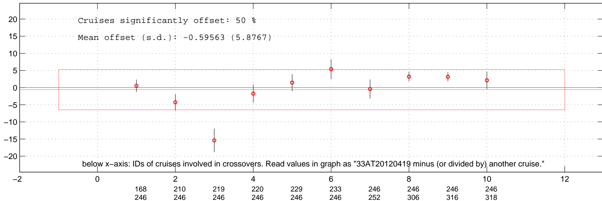
all additive offsets of ALK of 33AT20120419 in Favourite-space.
