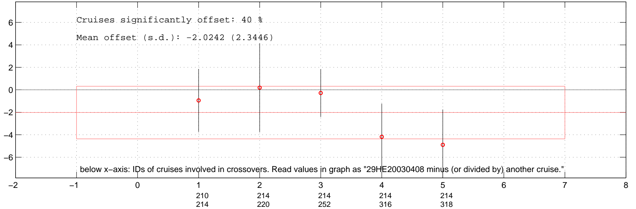
all multiplicative offsets of NO3 of 29HE20030408 in Favourite-space.
