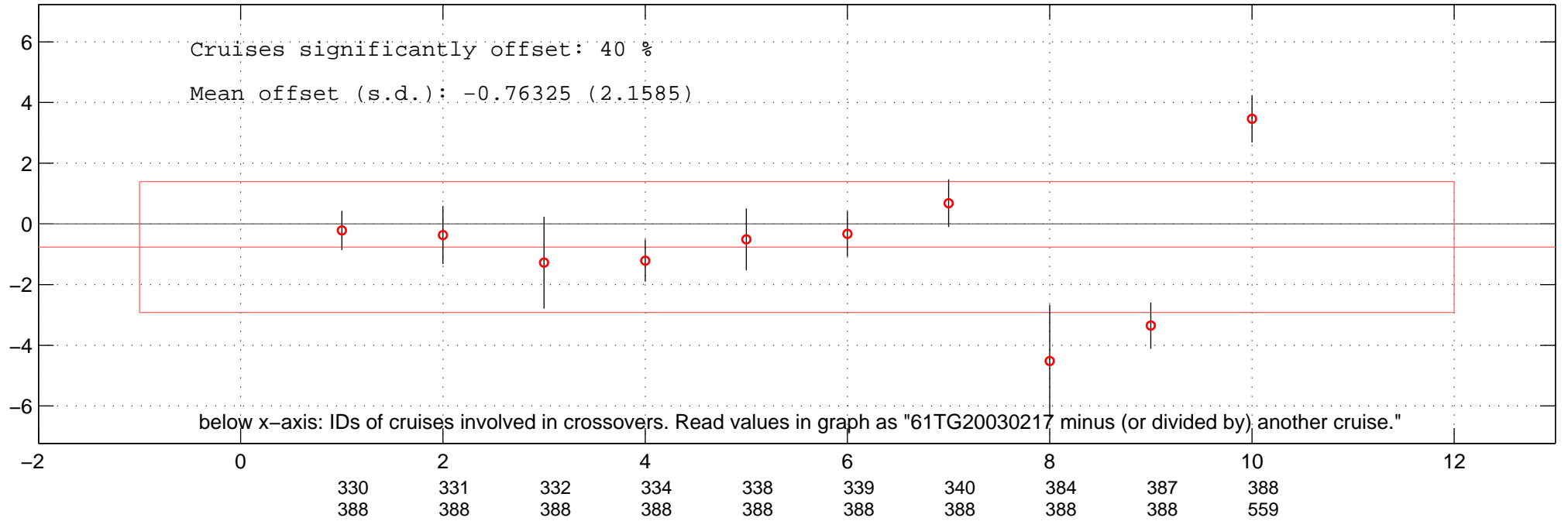
all multiplicative offsets of NO3 of 61TG20030217 in Favourite-space.
