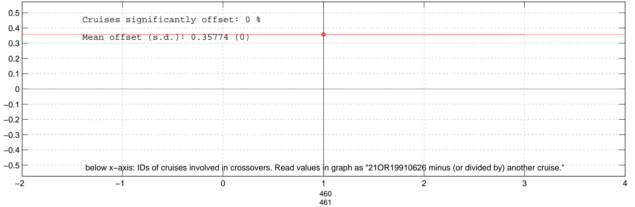
all multiplicative offsets of NO3 of 21OR19910626 in Favourite-space.
