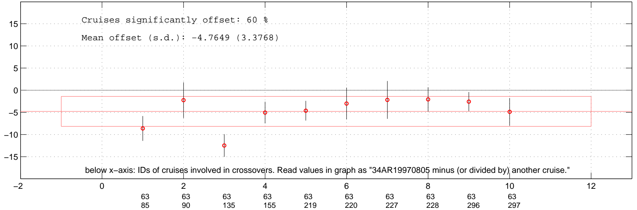
all multiplicative offsets of NO3 of 34AR19970805 in Favourite-space.
