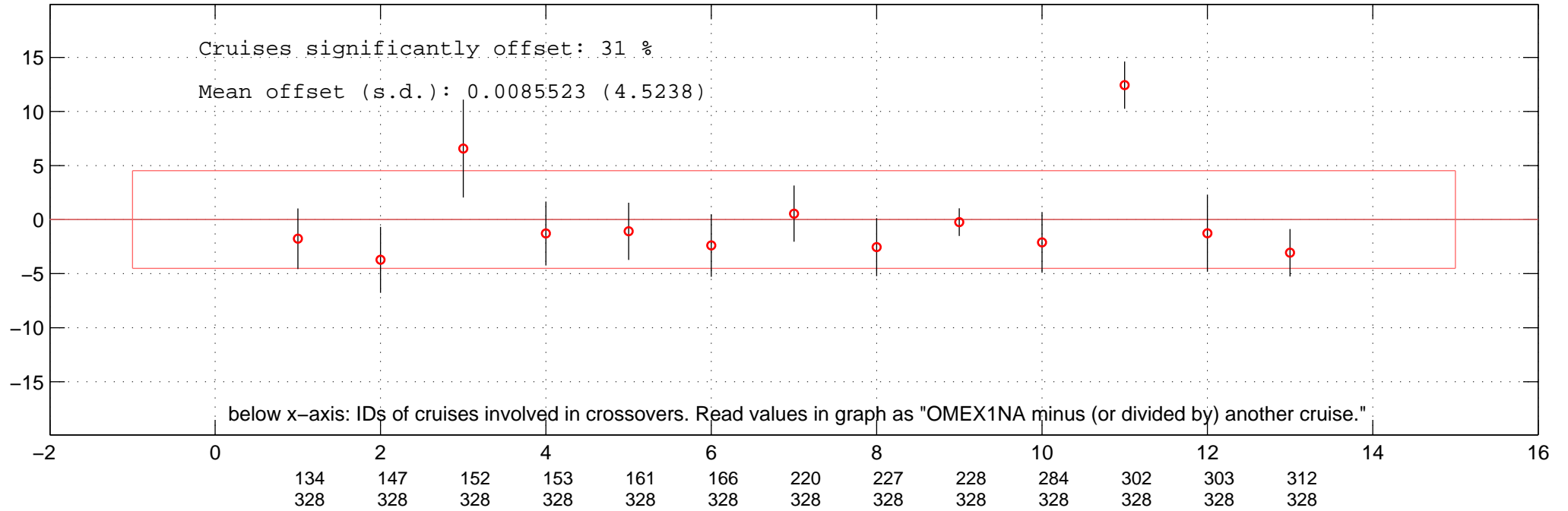
all multiplicative offsets of NO3 of OMEX1NA in Favourite-space.
