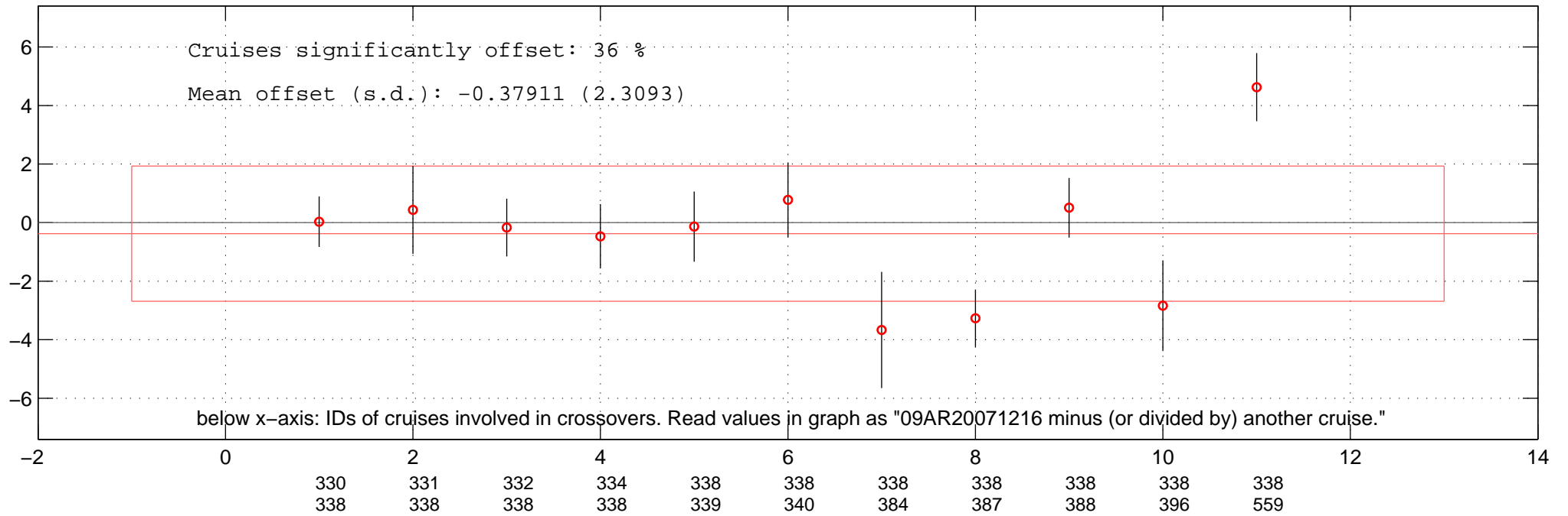
all multiplicative offsets of NO3 of 09AR20071216 in Favourite-space.
