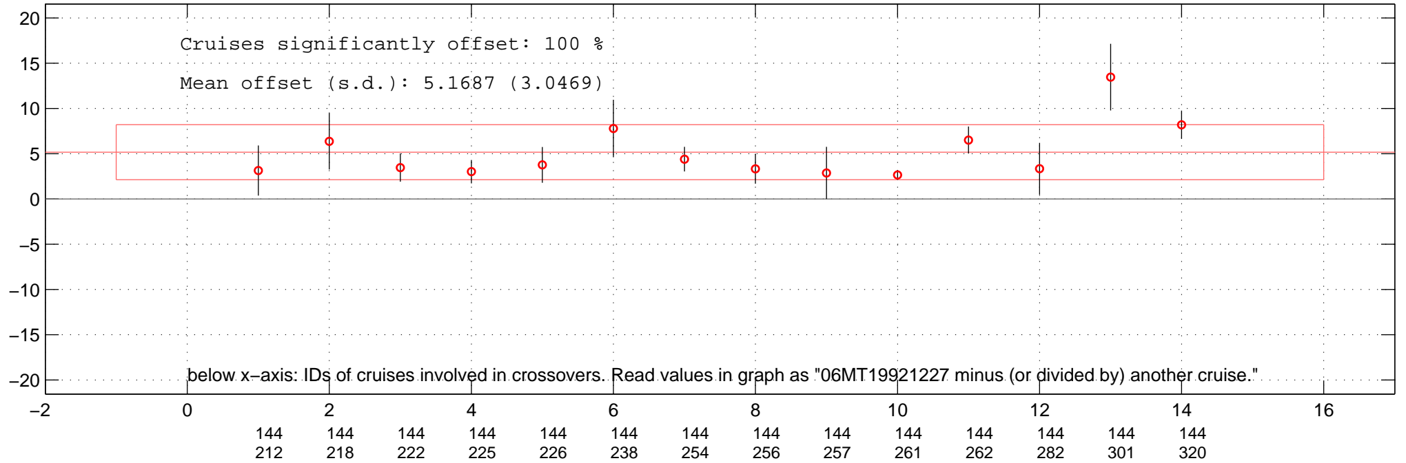
all multiplicative offsets of NO3 of 06MT19921227 in Favourite-space.
