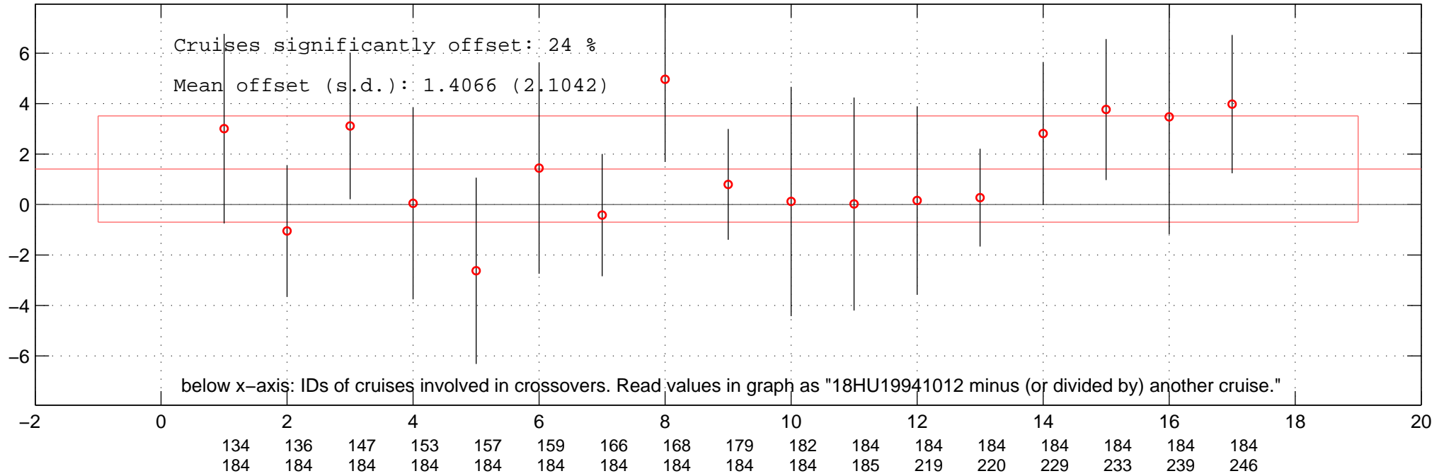
all multiplicative offsets of NO3 of 18HU19941012 in Favourite-space.
