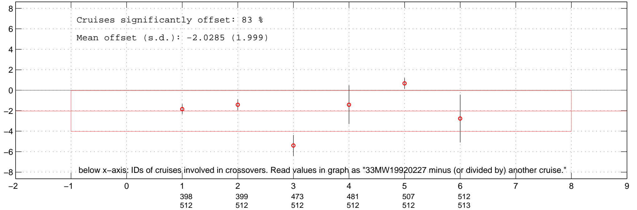
all multiplicative offsets of NO3 of 33MW19920227 in Favourite-space.
