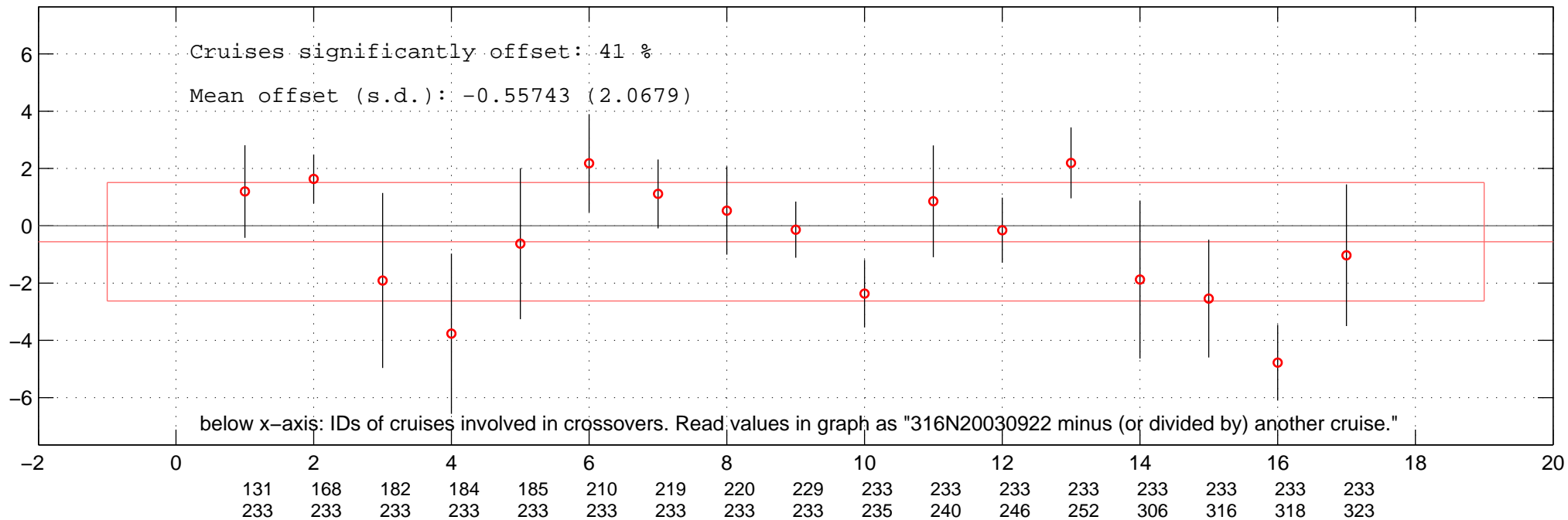
all multiplicative offsets of NO3 of 316N20030922 in Favourite-space.
