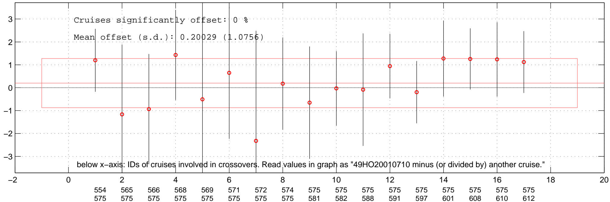
all multiplicative offsets of O2 of 49HO20010710 in Favourite-space.
