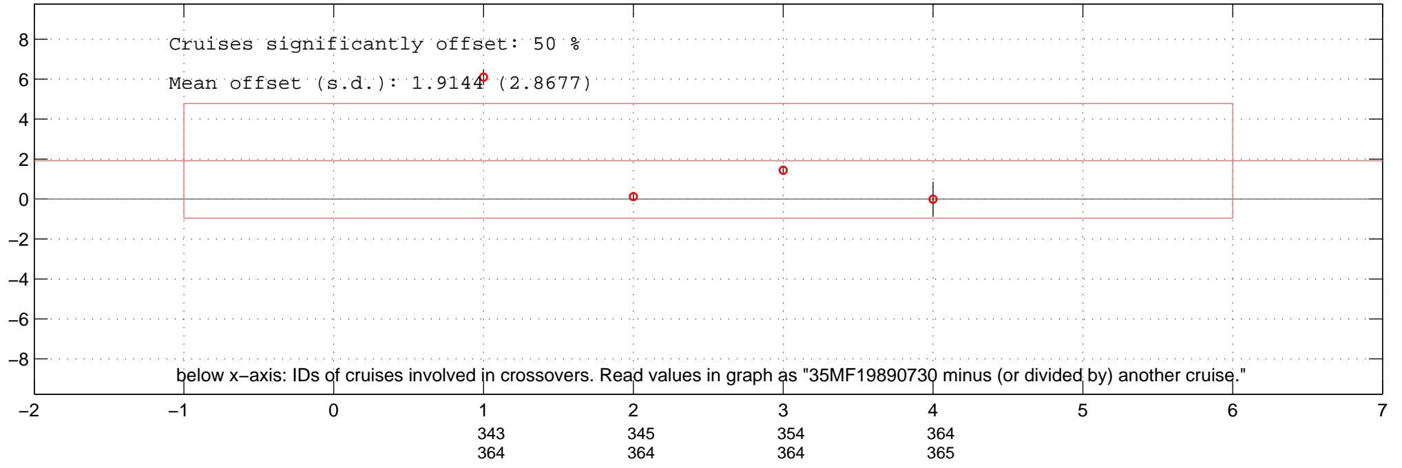
all multiplicative offsets of O2 of 35MF19890730 in Favourite-space.
