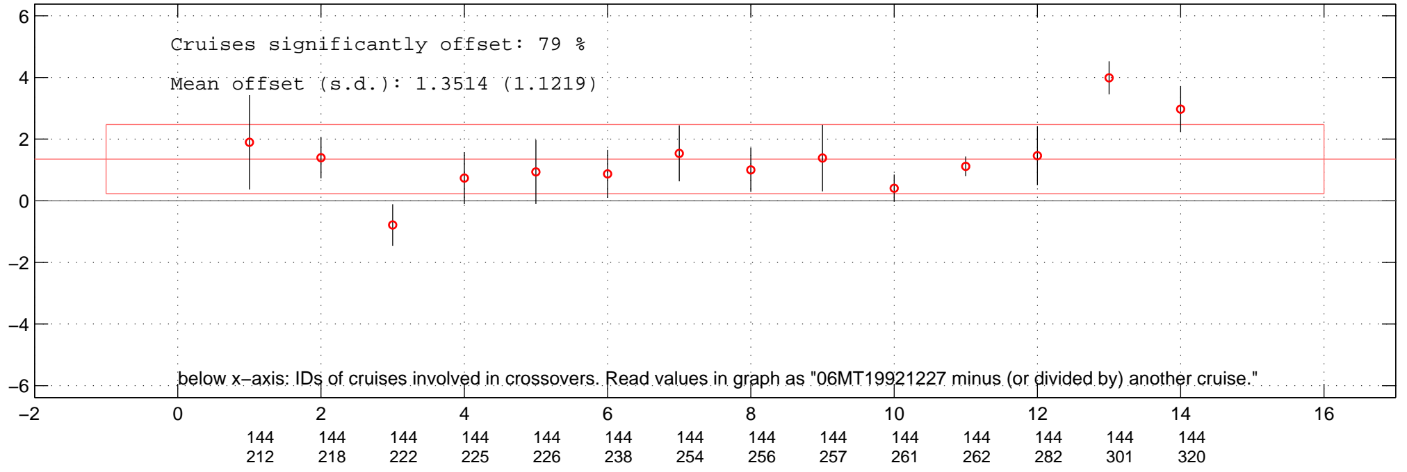
all multiplicative offsets of O2 of 06MT19921227 in Favourite-space.
