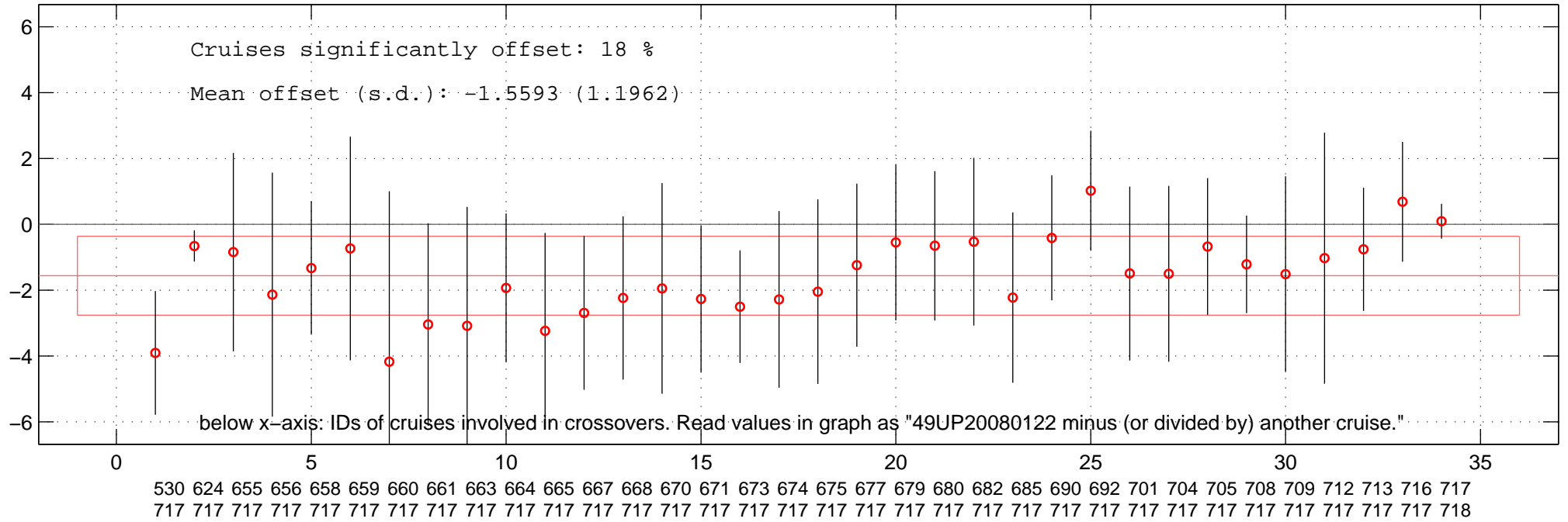
all multiplicative offsets of O2 of 49UP20080122 in Favourite-space.
