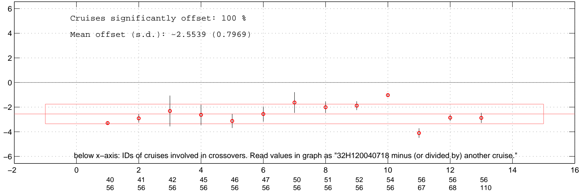
all multiplicative offsets of O2 of 32H120040718 in Favourite-space.
