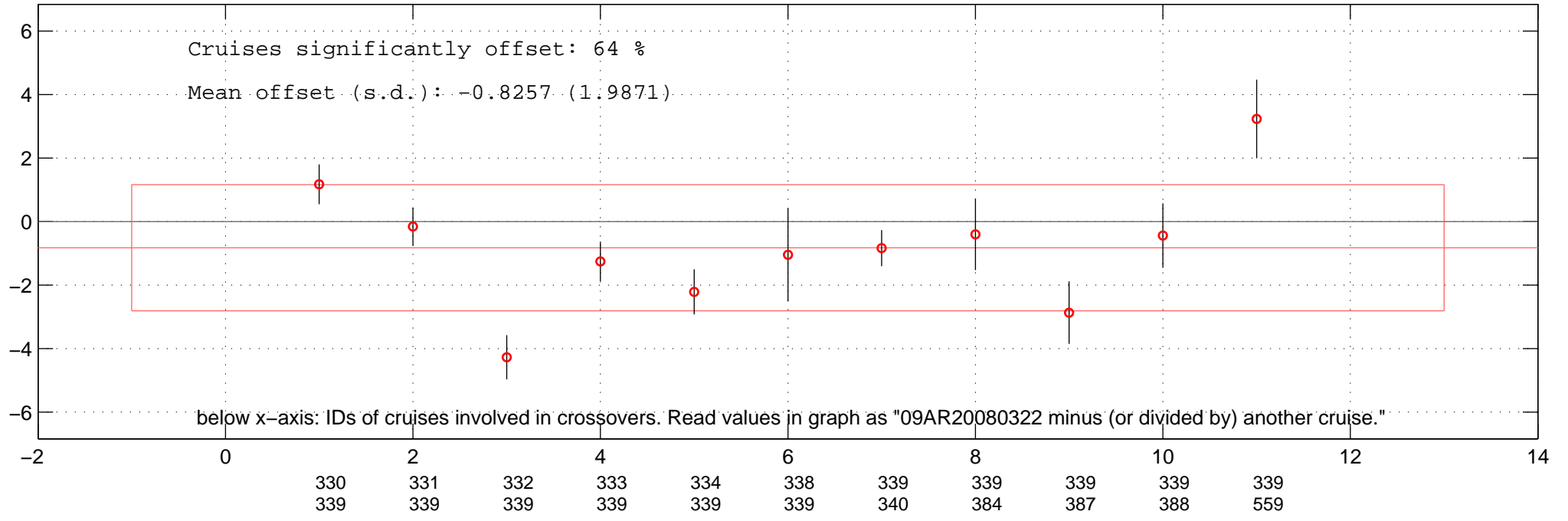
all multiplicative offsets of O2 of 09AR20080322 in Favourite-space.
