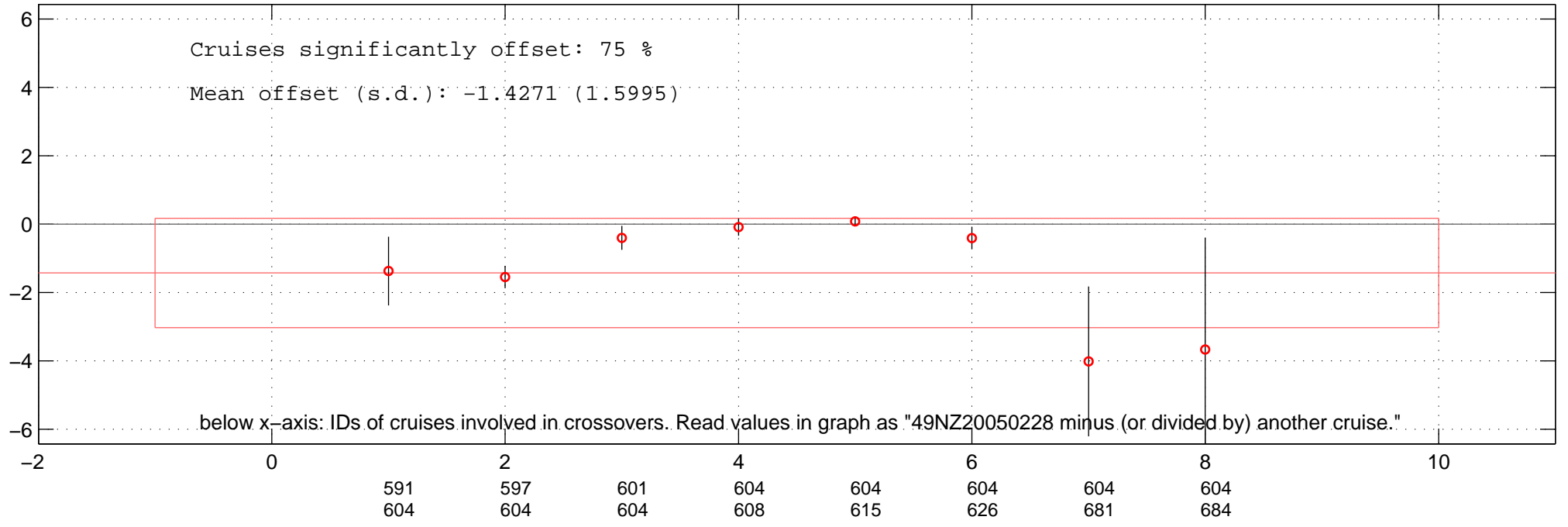
all multiplicative offsets of O2 of 49NZ20050228 in Favourite-space.
