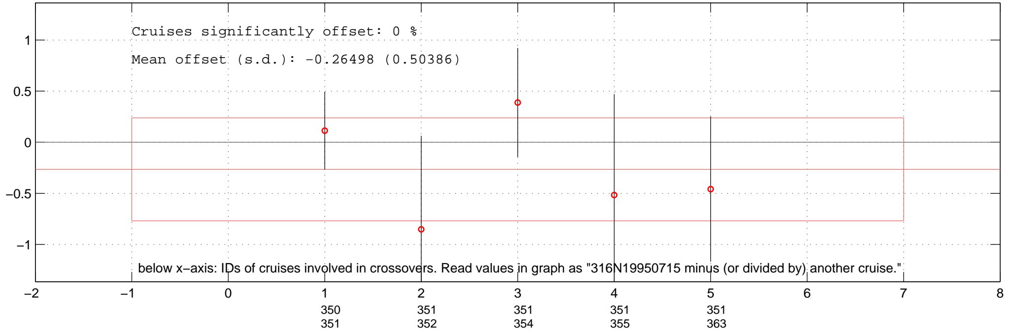
all multiplicative offsets of O2 of 316N19950715 in Favourite-space.
