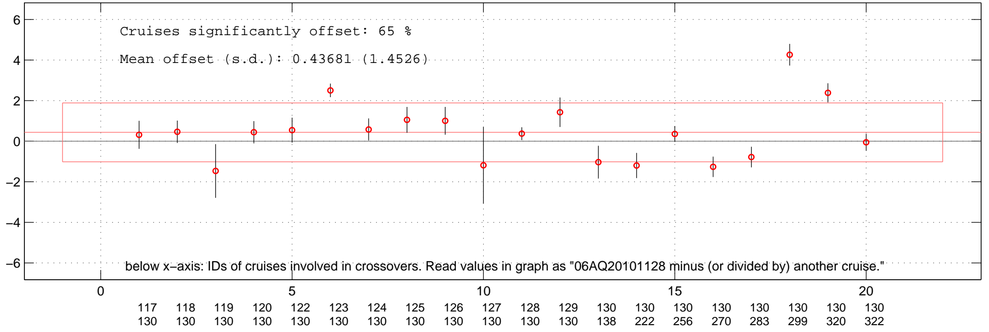
all multiplicative offsets of O2 of 06AQ20101128 in Favourite-space.
