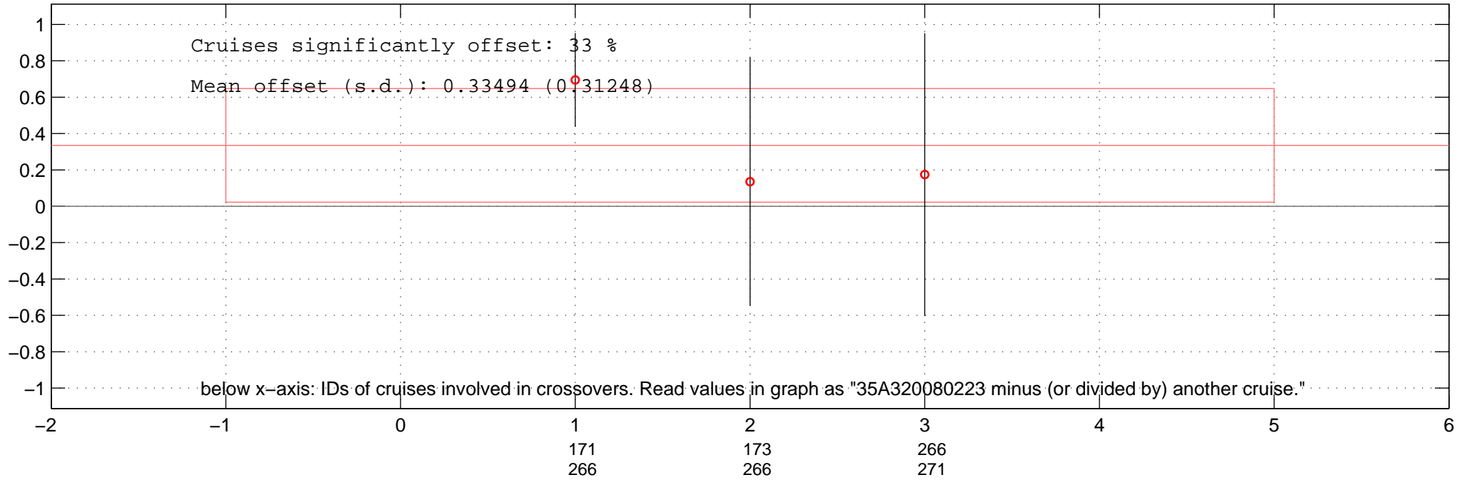
all multiplicative offsets of O2 of 35A320080223 in Favourite-space.
