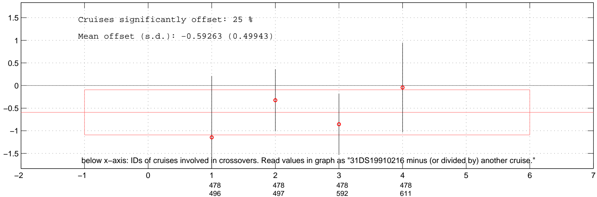
all multiplicative offsets of O2 of 31DS19910216 in Favourite-space.
