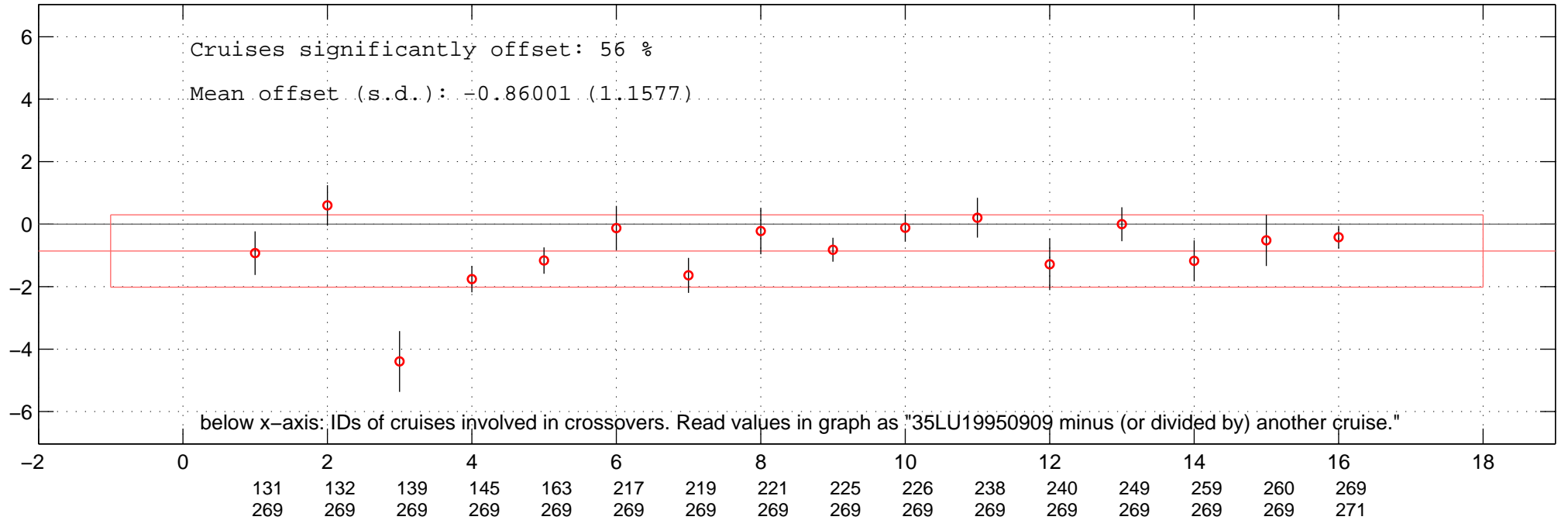
all multiplicative offsets of O2 of 35LU19950909 in Favourite-space.
