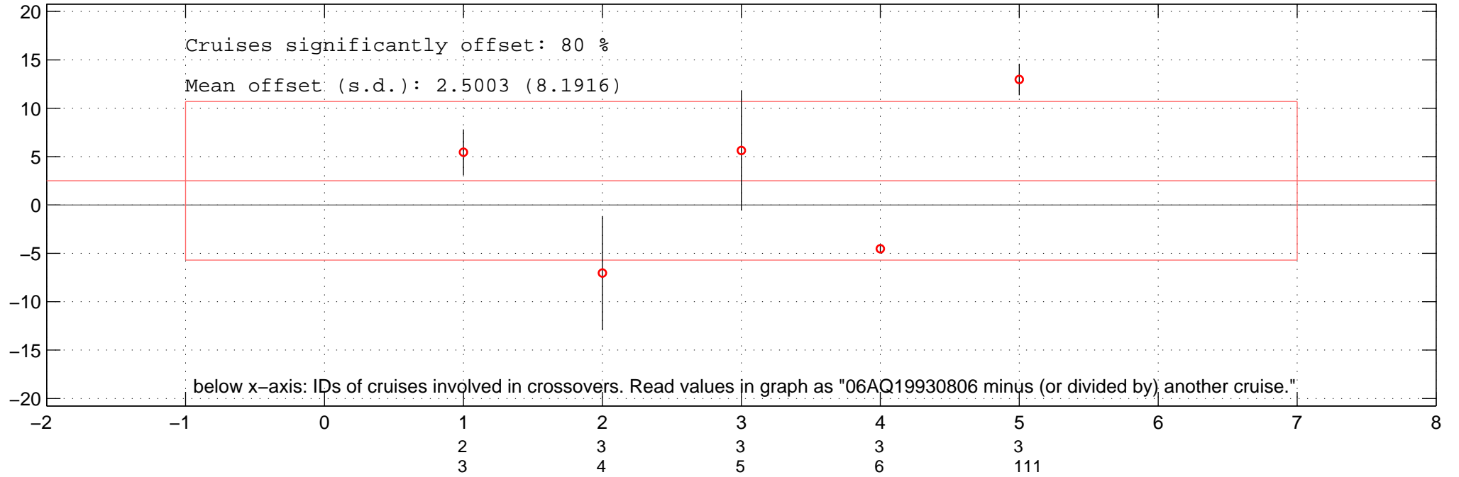
all multiplicative offsets of PO4 of 06AQ19930806 in Favourite-space.
