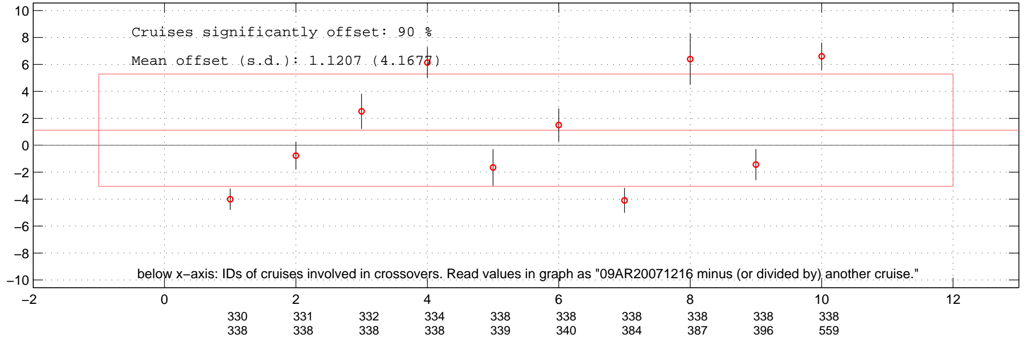
all multiplicative offsets of PO4 of 09AR20071216 in Favourite-space.
