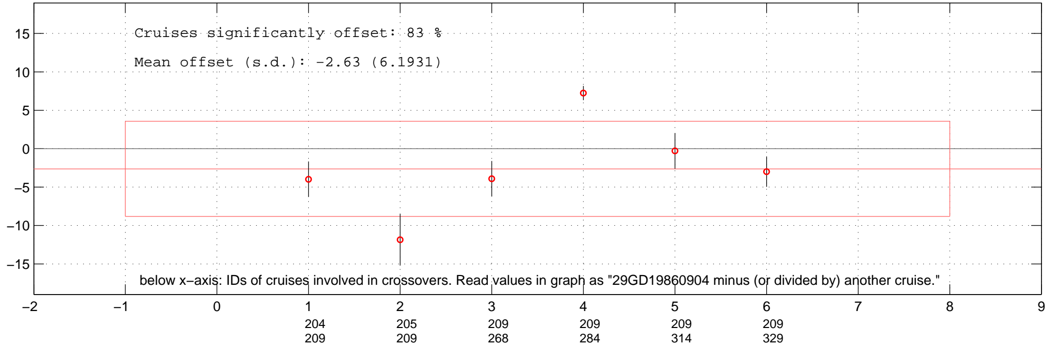
all multiplicative offsets of PO4 of 29GD19860904 in Favourite-space.
