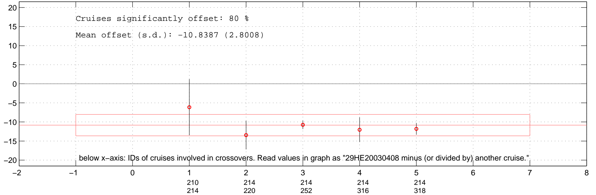
all multiplicative offsets of PO4 of 29HE20030408 in Favourite-space.
