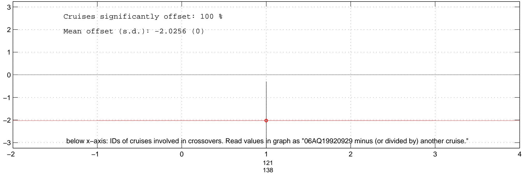
all multiplicative offsets of PO4 of 06AQ19920929 in Favourite-space.
