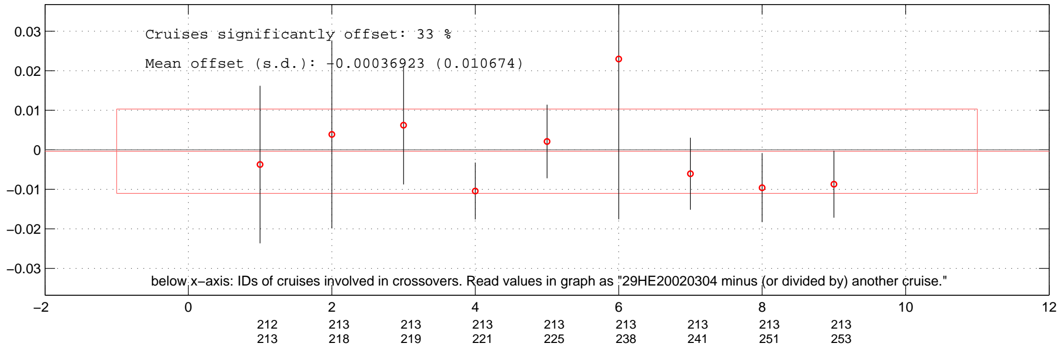
all additive offsets of SAL of 29HE20020304 in Favourite-space.
