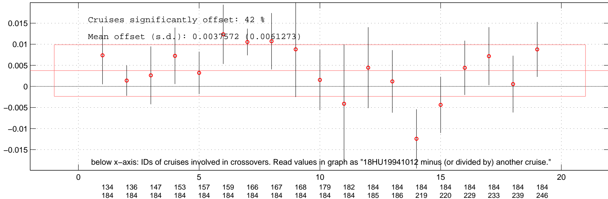
all additive offsets of SAL of 18HU19941012 in Favourite-space.
