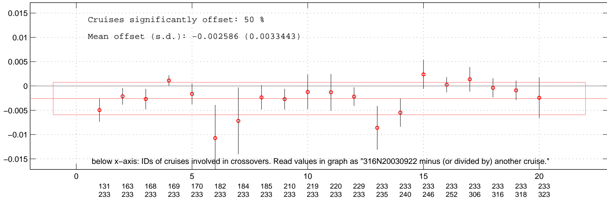
all additive offsets of SAL of 316N20030922 in Favourite-space.
