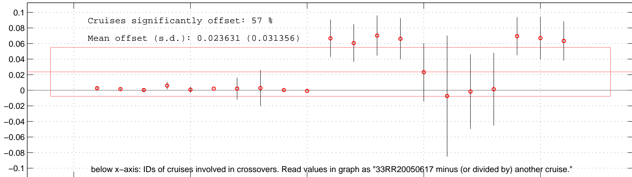
all additive offsets of SAL of 33RR20050617 in Favourite-space.
