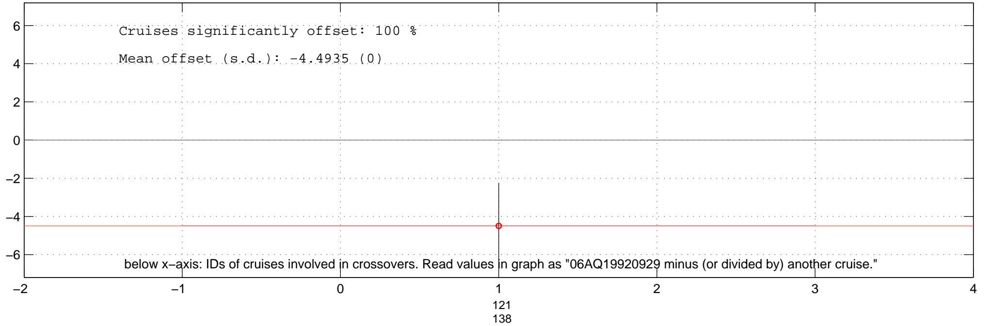
all multiplicative offsets of SIL of 06AQ19920929 in Favourite-space.
