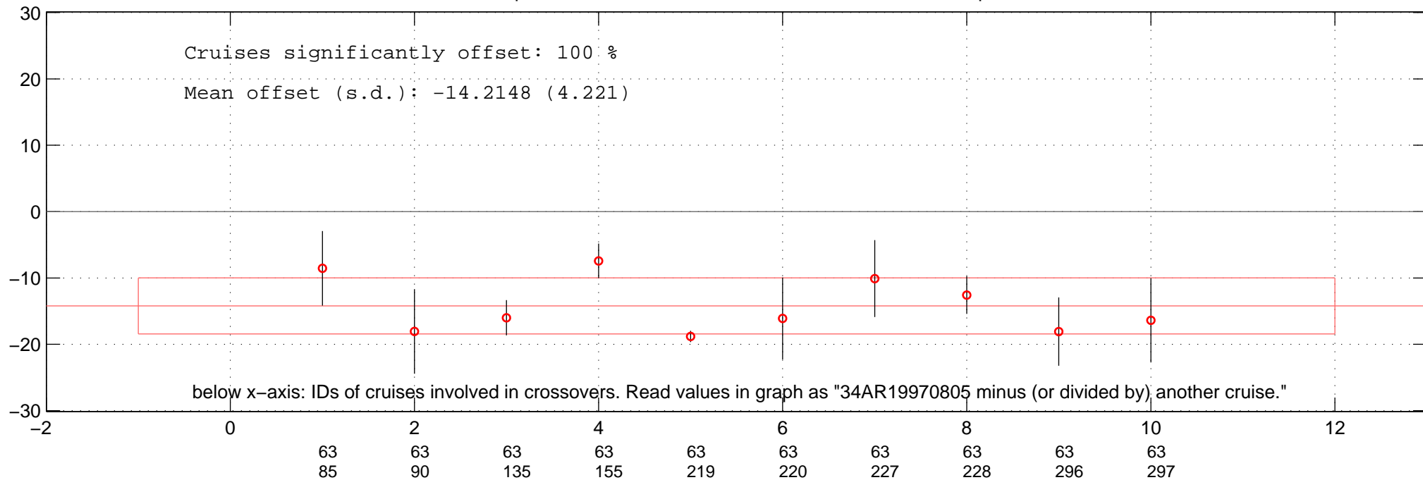
all multiplicative offsets of SIL of 34AR19970805 in Favourite-space.
