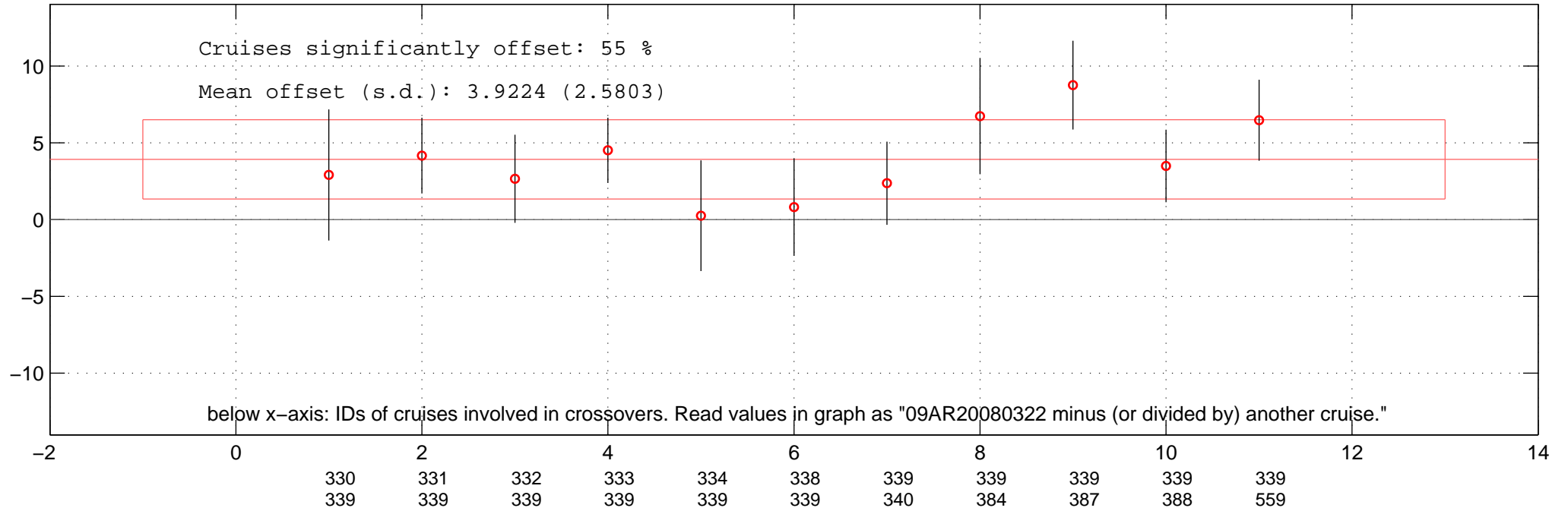
all multiplicative offsets of SIL of 09AR20080322 in Favourite-space.
