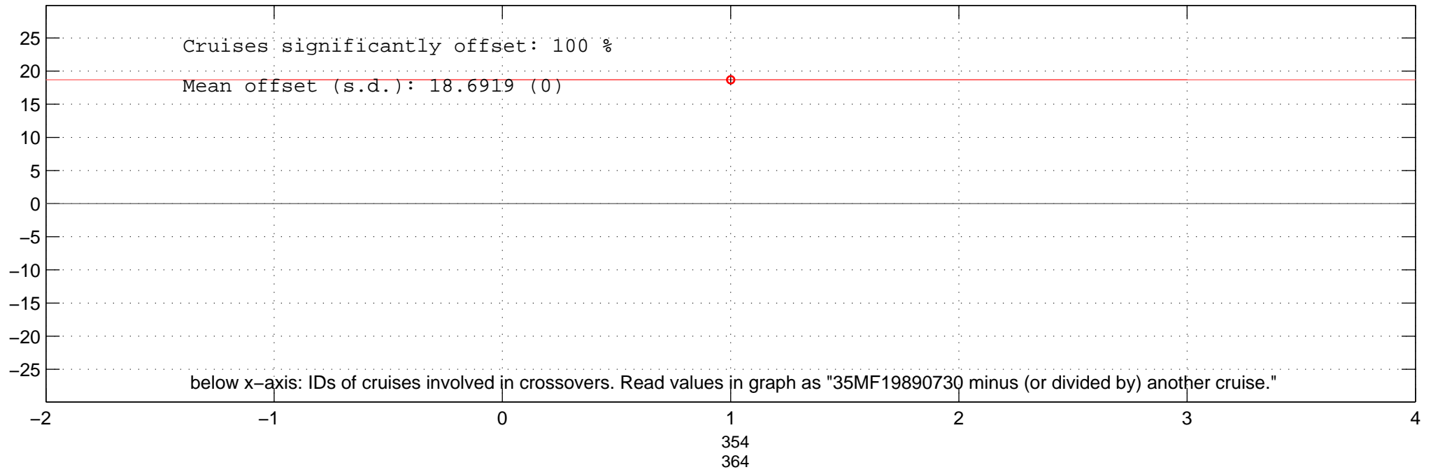
all additive offsets of DIC of 35MF19890730 in Favourite-space.
