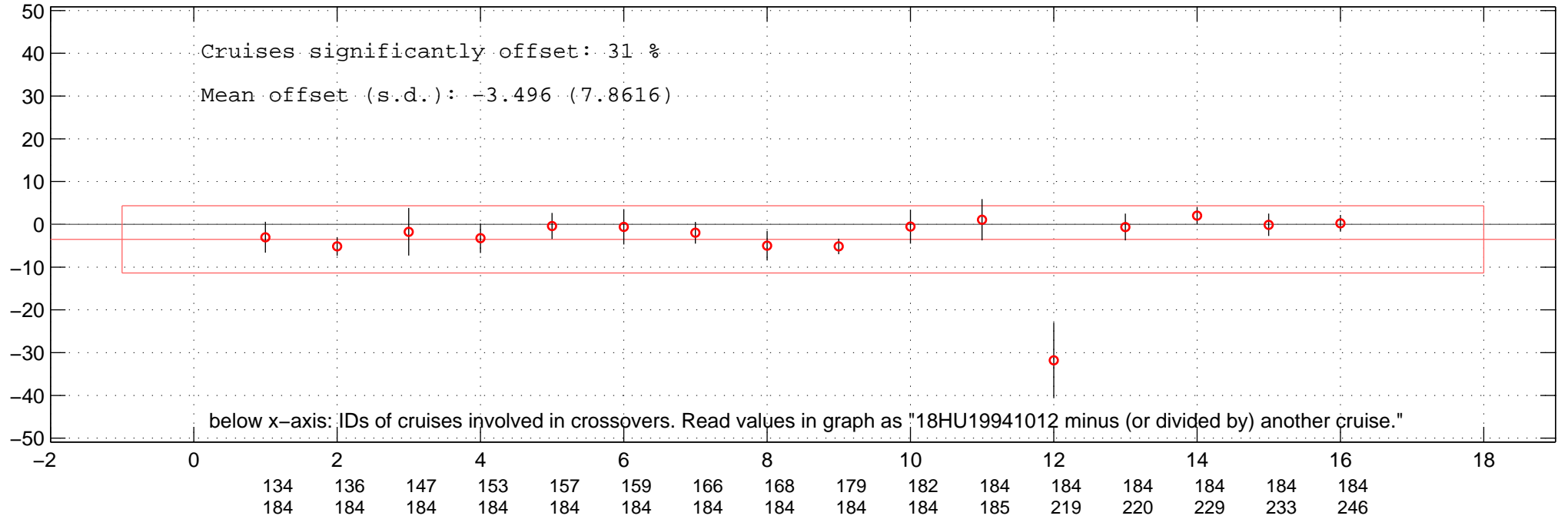
all additive offsets of DIC of 18HU19941012 in Favourite-space.
