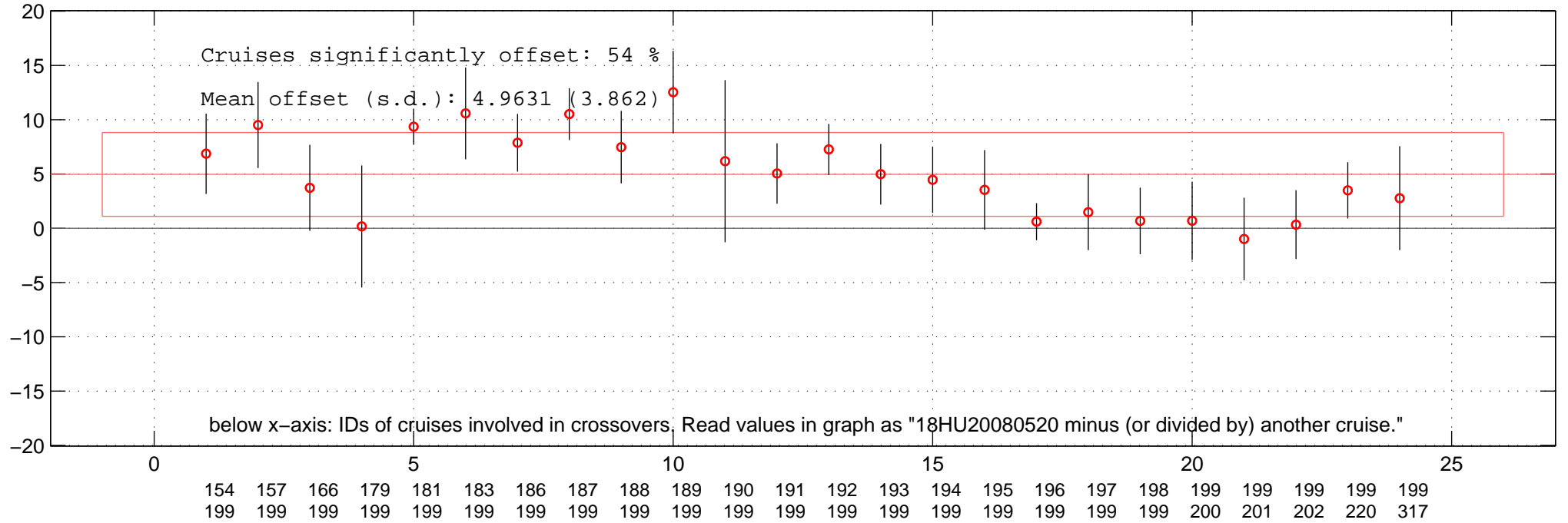
all additive offsets of DIC of 18HU20080520 in Favourite-space.
