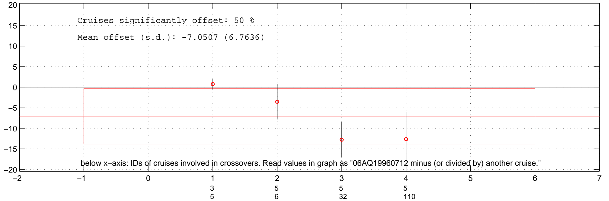
all additive offsets of DIC of 06AQ19960712 in Favourite-space.
