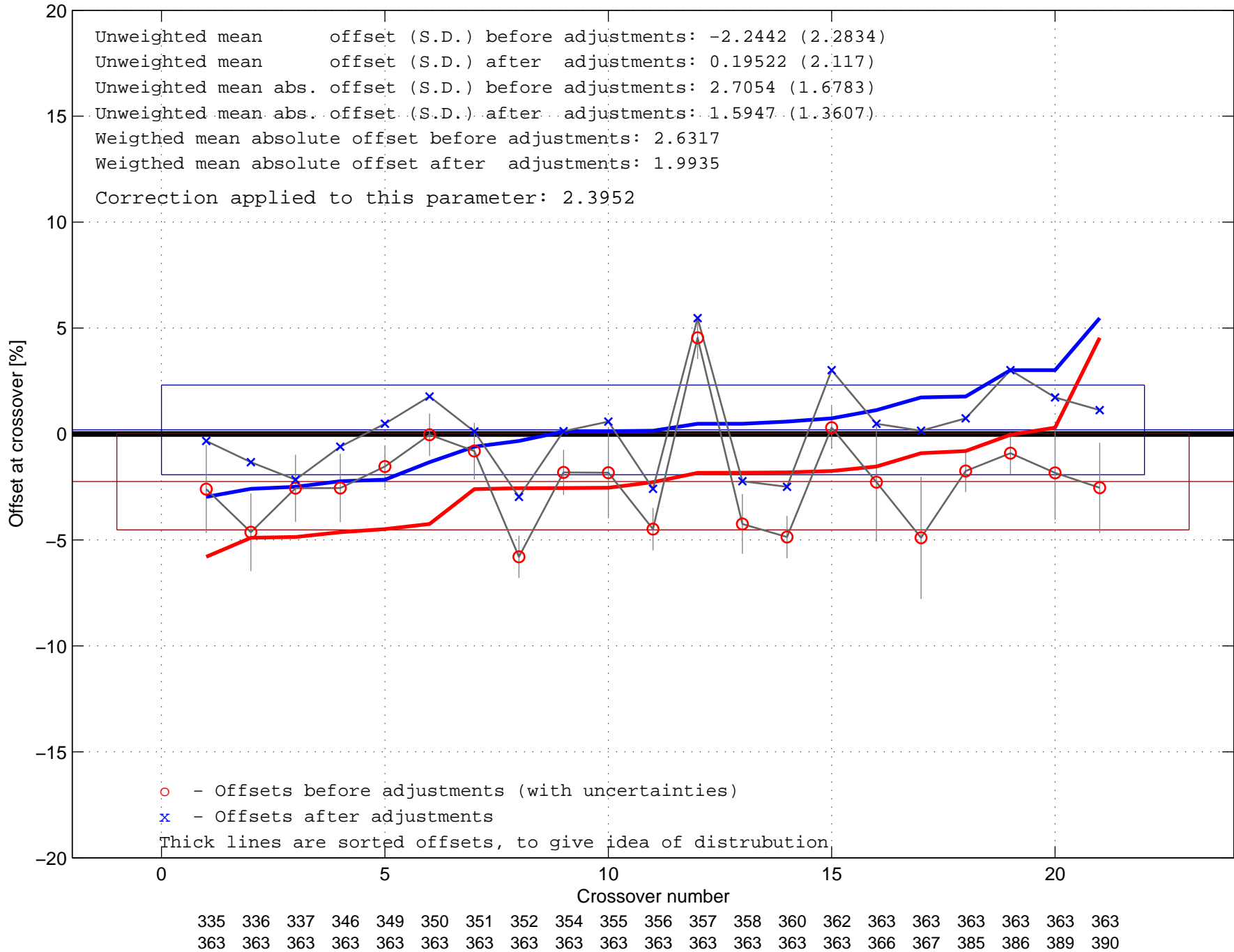
Multiplicative offsets for NO 3 for 35MF19850224 in Fav-space before (red) and after (blue) adjustment
