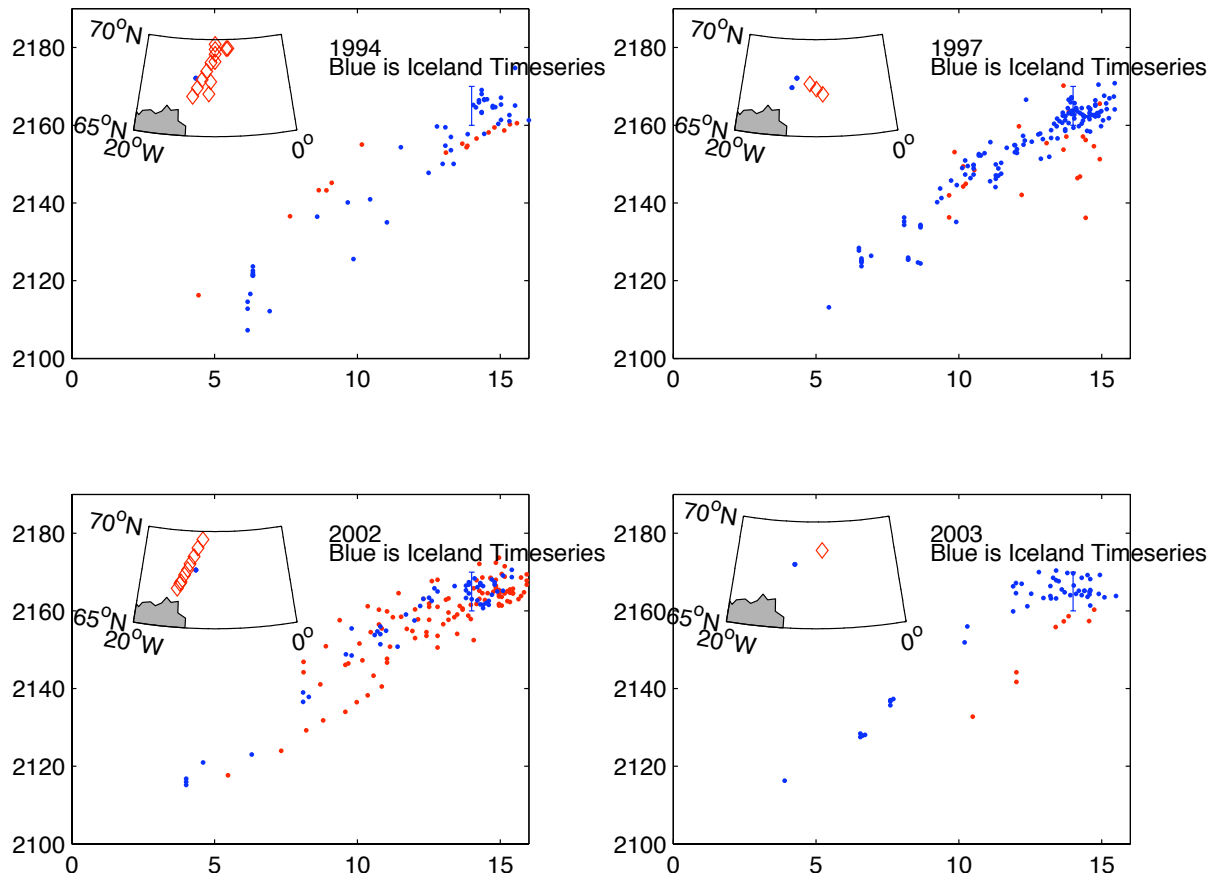
Figure 9. tco2 vs. nitrate for Iceland time series (blue) and cruise data (red).
