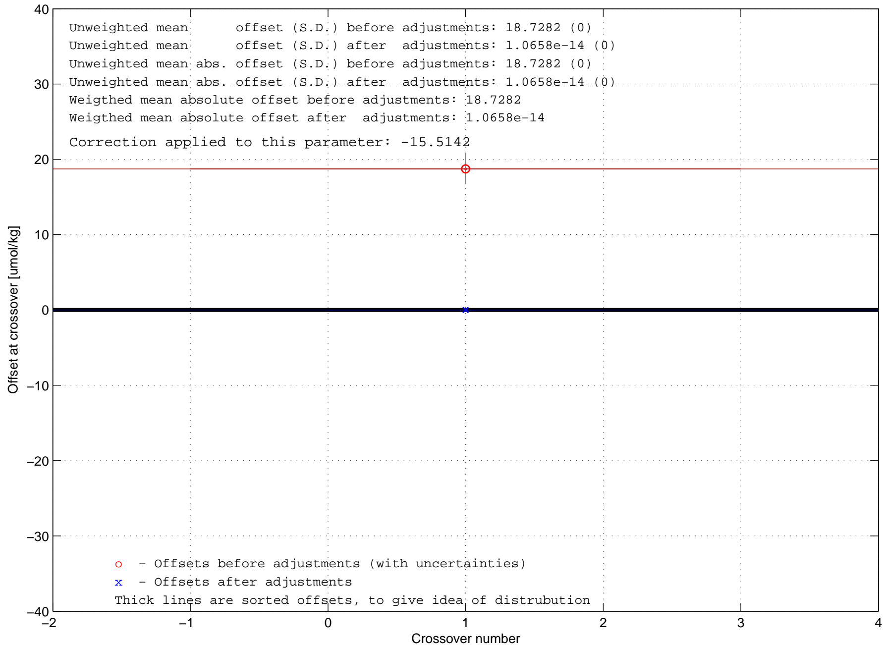
Additive offsets for TCO 2 for 35MF19890730 in Fav-space before (red) and after (blue) correction
