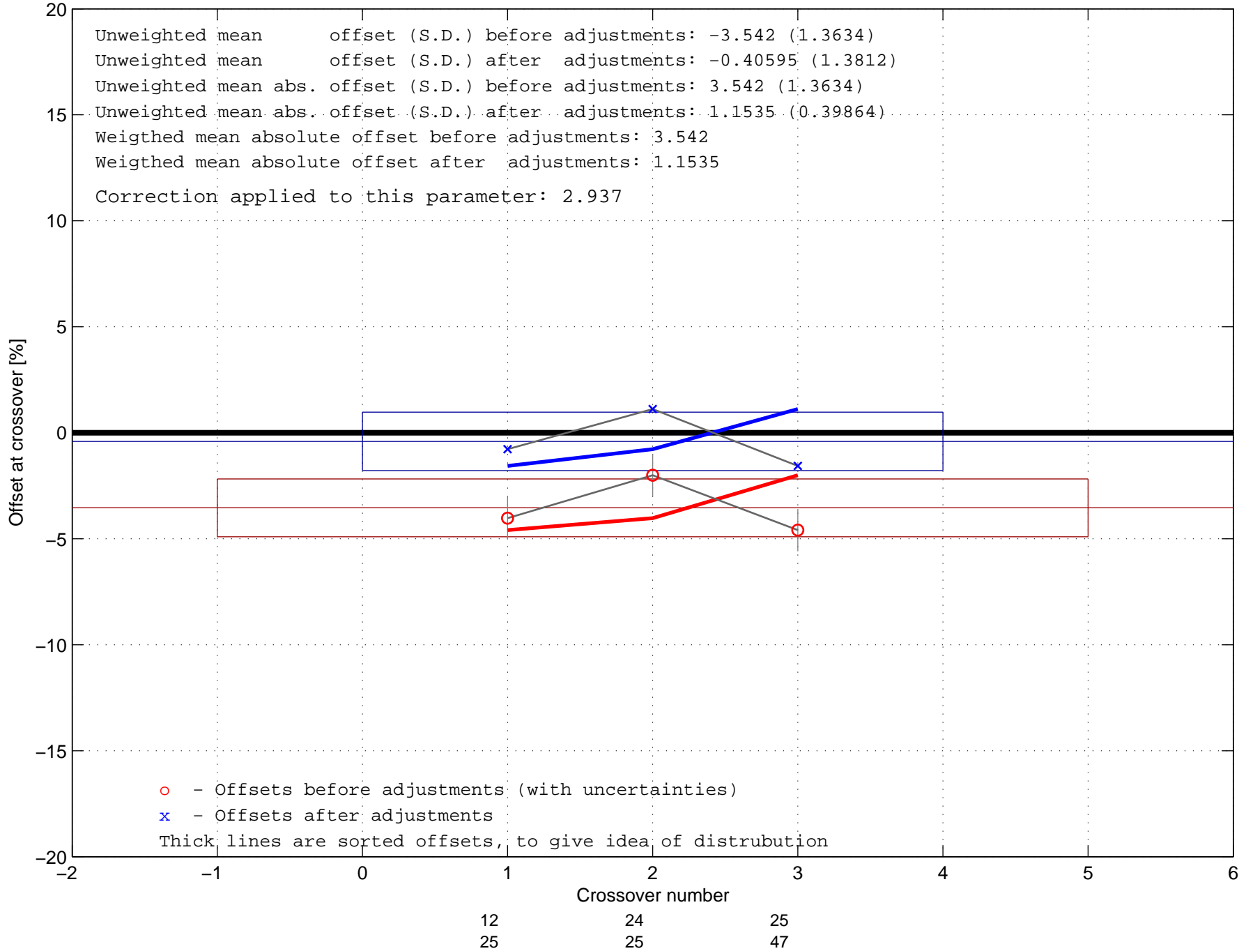
Multiplicative offsets for Si for 35MF19890730 in Fav-space before (red) and after (blue) correction
